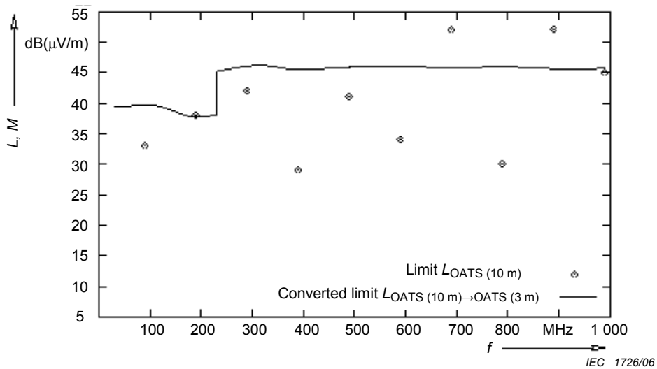
Figure B.25 – Comparison of the corrected values with the converted limit
