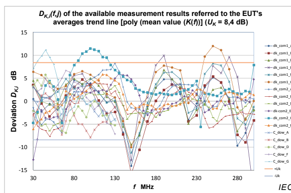
Figure C.9 – Deviation of the conversion factors from the trend line [poly (mean value K(f) )] ( U_K = 8,4 dB)
