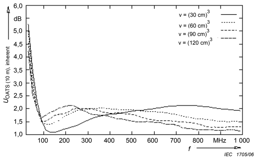
Figure B.7 – Uncertainties due to the unknown EUT characteristic for 3 m FAR (top) and 10 m OATS (bottom)
